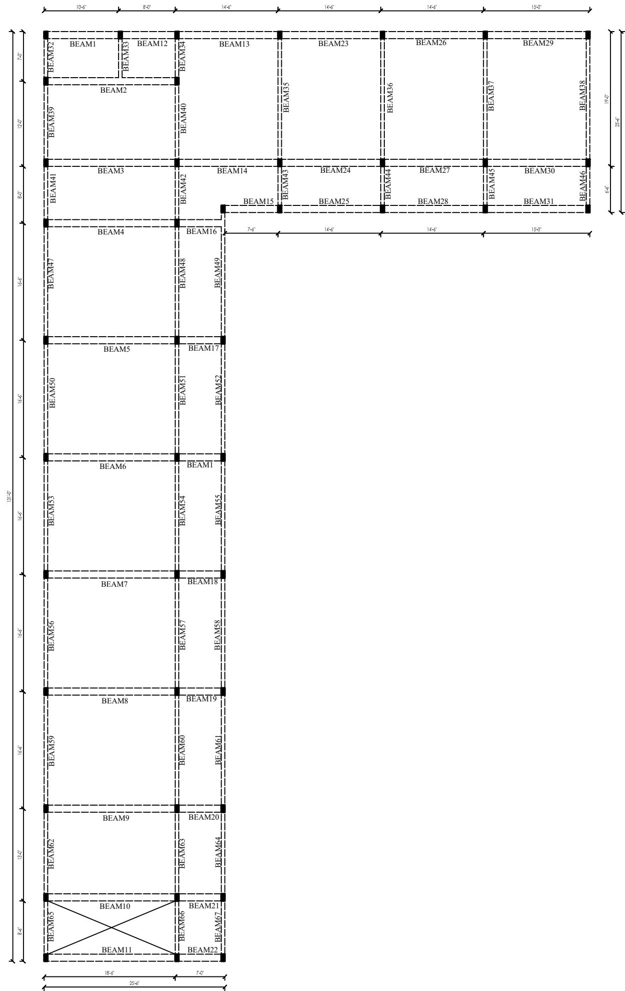
(A) BEAM LAYOUTS
