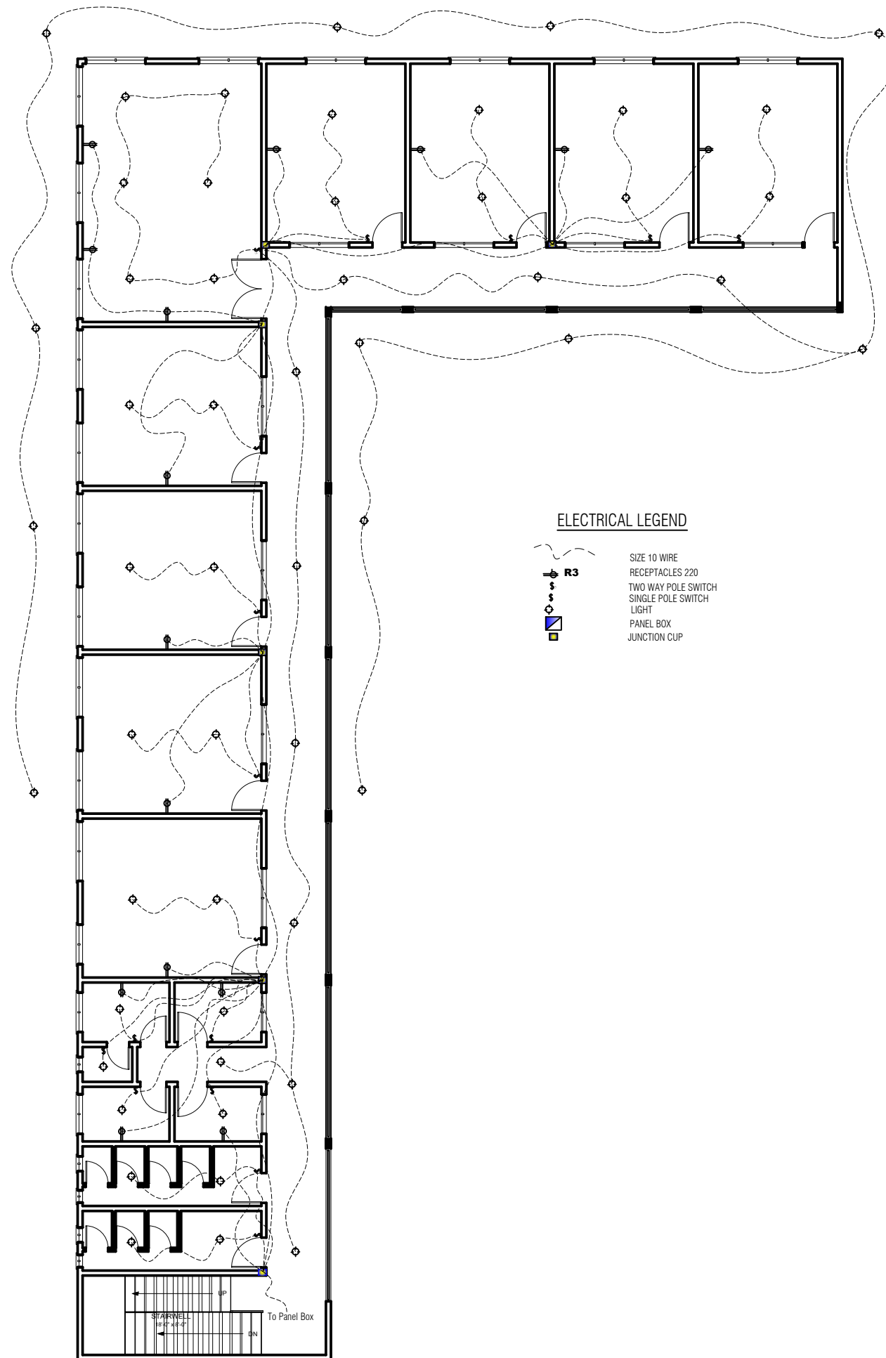
PROPOSE FIRST FLOOR ELECTRICAL PLAN
