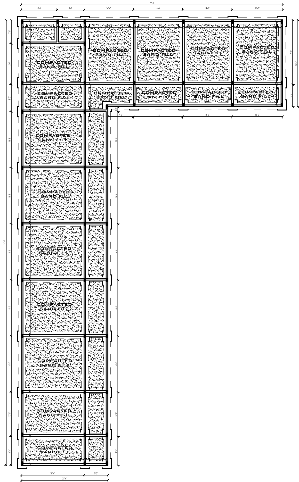
PROPOSE FOUNDATION PLAN LIVING AREA 4653 sq ft
