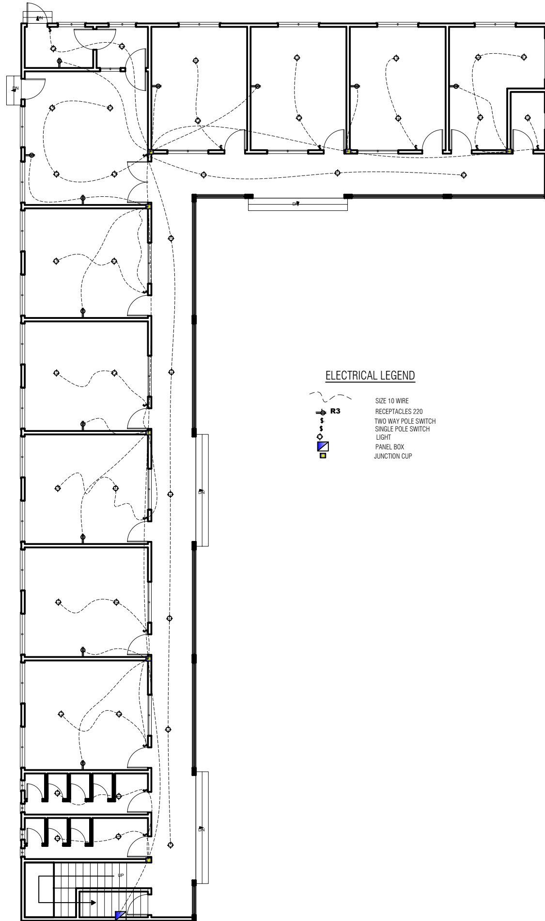
A PROPOSE GROUND FLOOR ELECTRICAL PLAN
