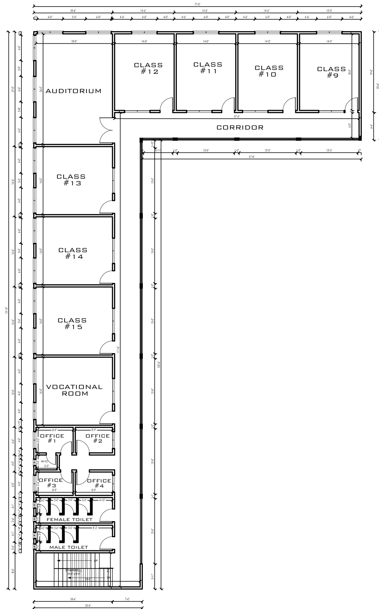
PROPOSE FIRST FLOOR PLAN LIVING AREA 4503 SQ FT
